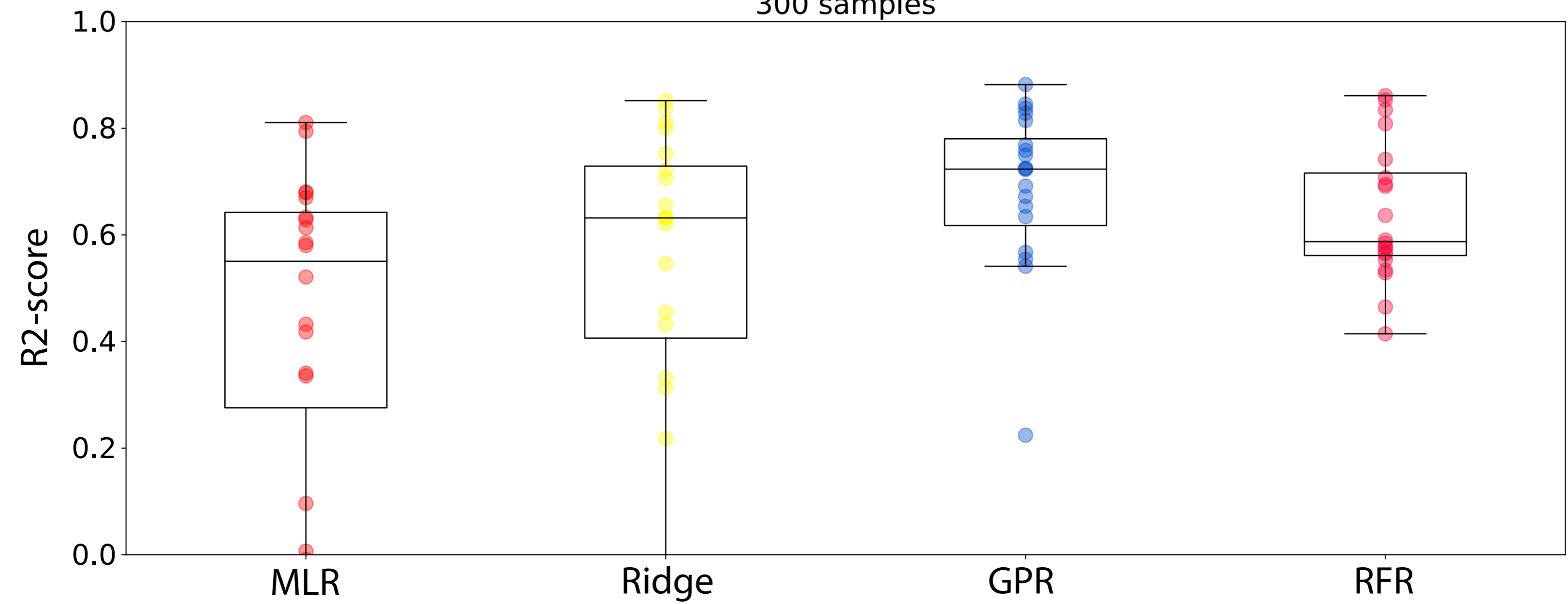
300 samples
