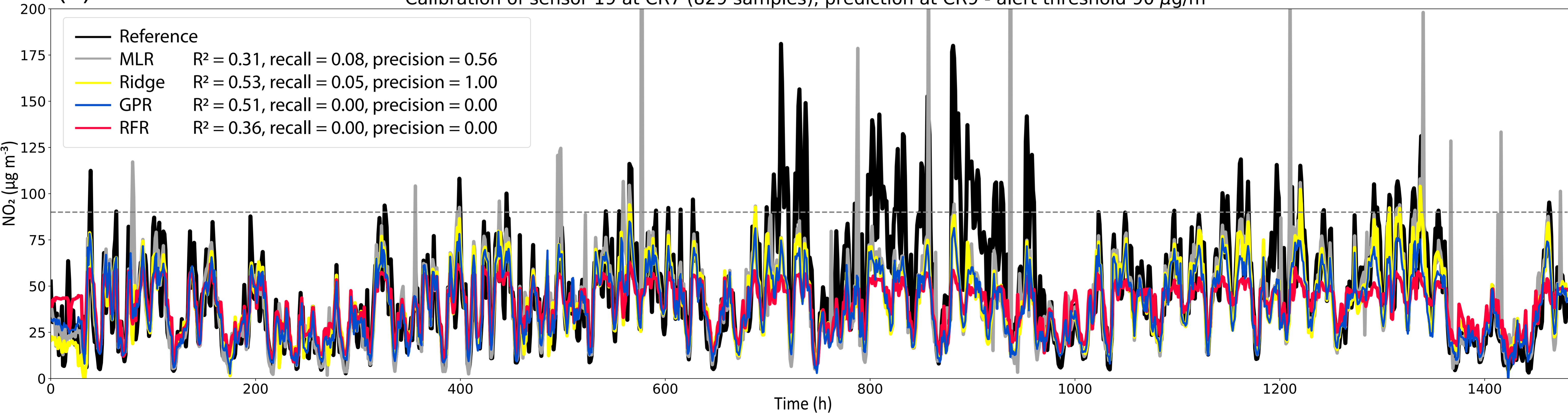
Calibration of sensor 19 at CR7 (829 samples), prediction at CR9 - alert threshold 90 \mu\text{g}/\text{m}^3
