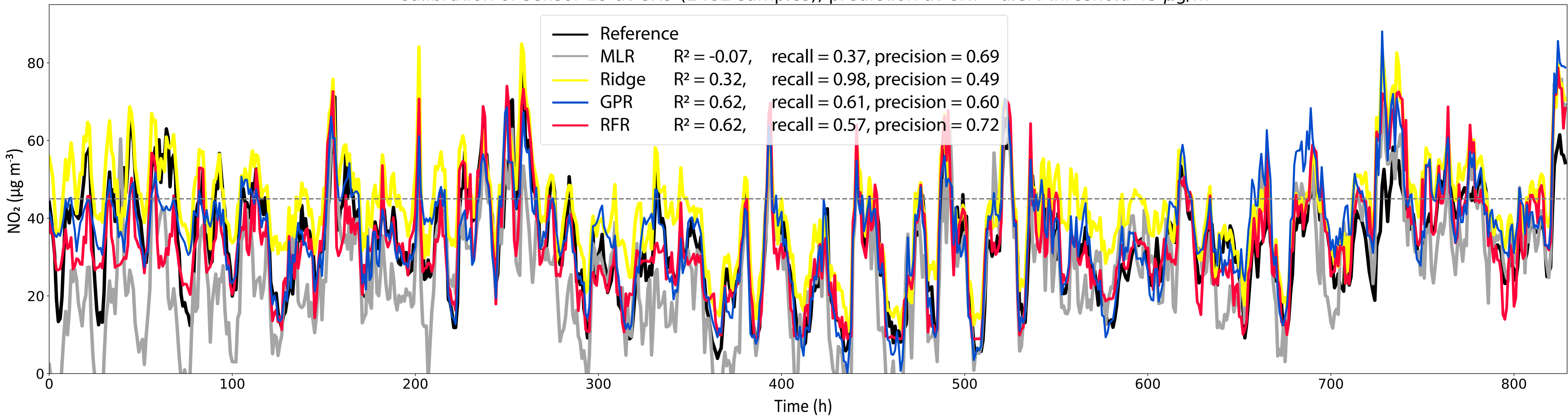
Calibration of sensor 19 at CR9 (1482 samples), prediction at CR7 - alert threshold 45 \mu\text{g}/\text{m}^3
