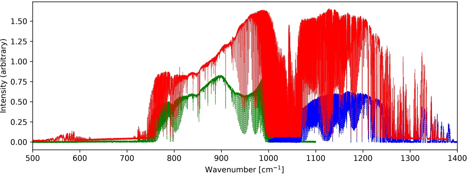
FTIR spectra at Syowa Station
