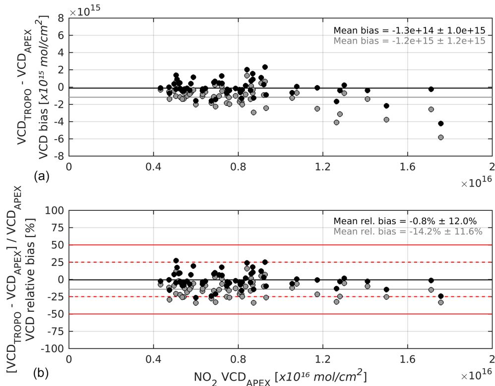
Figure 9. (a) NO 2 VCD bias ( VCD_{\text{TROPO}(-\text{CRE})} - VCD_{\text{APEX}} ) and (b) NO 2 VCD relative bias ( (VCD_{\text{TROPO}(-\text{CRE})} - VCD_{\text{APEX}}) / VCD_{\text{APEX}} \cdot 100 ) for the ensemble of the four data sets, acquired during the S5PVAL-BE campaign. Data points and statistics are colour coded grey and black for the comparison of TM5-MP-based and CAMS-based TROPOMI VCD retrievals with APEX, respectively, in analogy to Fig. 8. The grey and black horizontal lines represent the average (relative) bias. The dashed red and full horizontal lines represent the 25 % and 50 % bias between coincident TROPOMI and APEX NO 2 VCDs, respectively.
