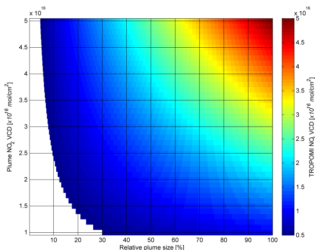
Figure 15. Simulations of NO 2 VCDs based on an isolated NO 2 hotspot surrounded by urban background pixels (3 × 10 15 molec cm -2 ). The NO 2 hotspot is defined by its relative size on the x axis, expressed as the fraction of a 3.5 km by 5.5 km TROPOMI nadir pixel, and average NO 2 signal strength on the y axis. The separation between the white area and synthetic NO 2 VCDs corresponds to the hotspot detection threshold of 5.1 × 10 15 molec cm -2 .
