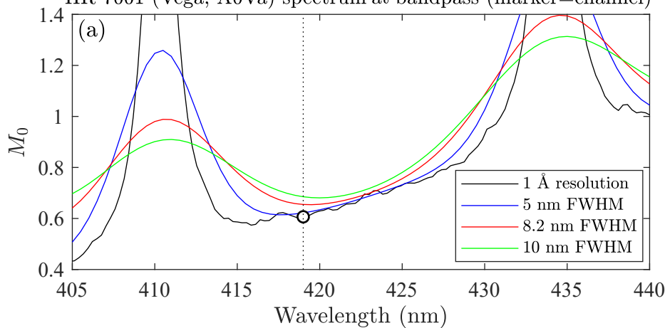
HR 7001 (Vega, A0Va) spectrum at bandpass (marker=channel)
