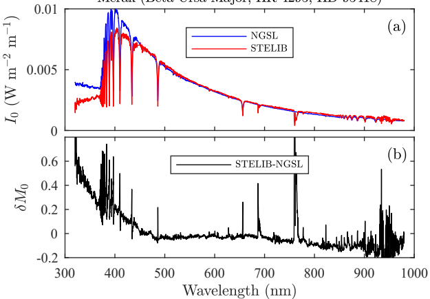
Merak (Beta Ursa Major, HR 4295, HD 95418)
