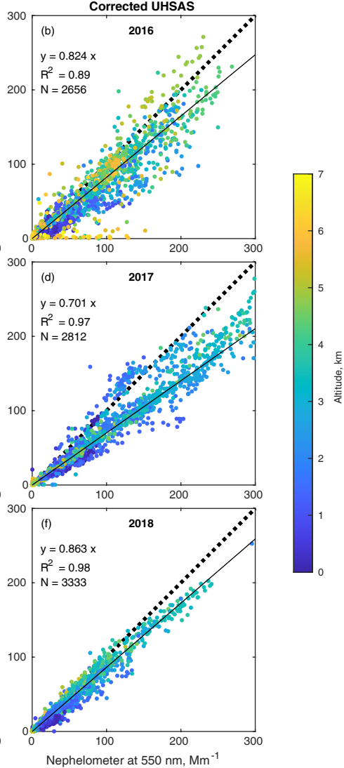
Corrected UHSAS
