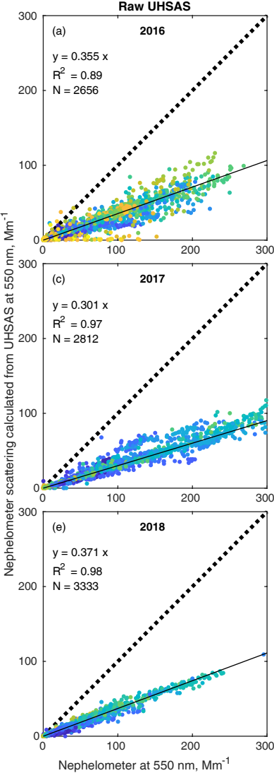
Raw UHSAS
