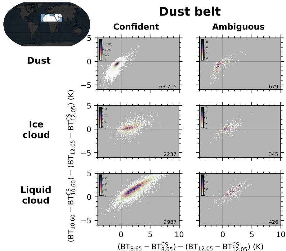
Figure 9. As Fig. 2 for dust, ice clouds, and liquid clouds detected in the dust belt region ( 10\text{--}38^\circ\text{ N} and 25^\circ\text{ W--}65^\circ\text{ E} ) with 4 < z_{\text{top}} < 8\text{ km} and 0.2 < \tau < 3 .
