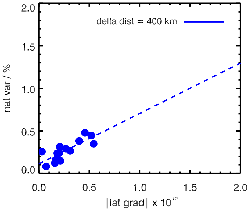
H 2 O in WACCM in AUTUMN at 30 km
