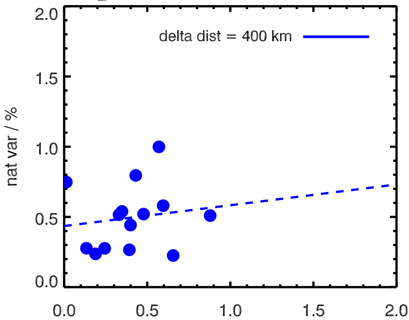
H 2 O in WACCM in AUTUMN at 30 km
