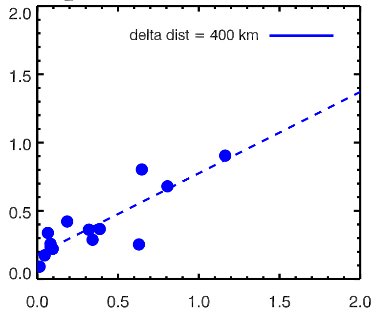
H 2 O in WACCM in WINTER at 30 km
