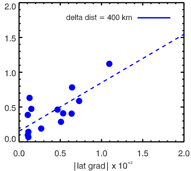
H 2 O in WACCM in WINTER at 30 km
