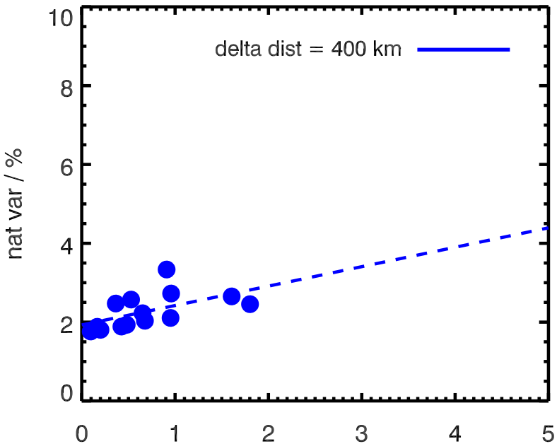
NO in WACCM in AUTUMN at 40 km
