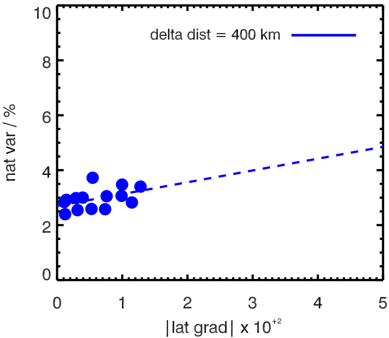
NO in WACCM in AUTUMN at 40 km
