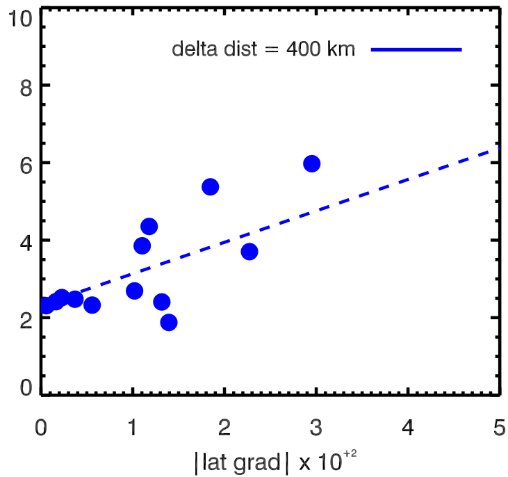
NO in WACCM in WINTER at 40 km
