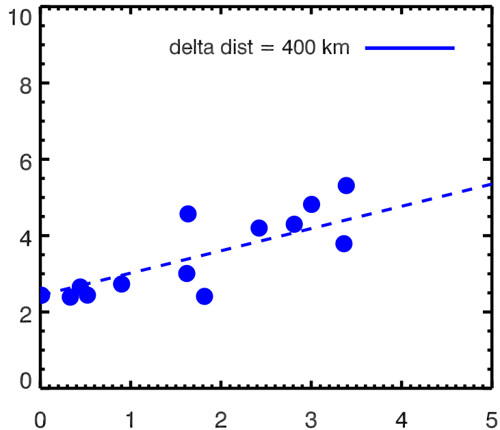
NO in WACCM in WINTER at 40 km
