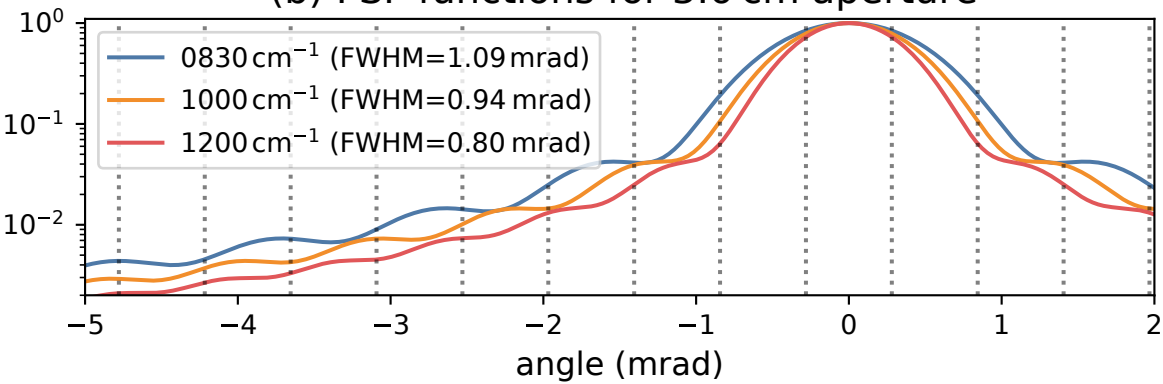
(b) PSF functions for 3.6 cm aperture
