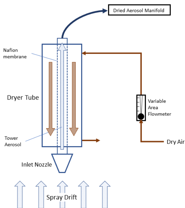
Figure 4. Configuration for a single MD-700 dryer.
