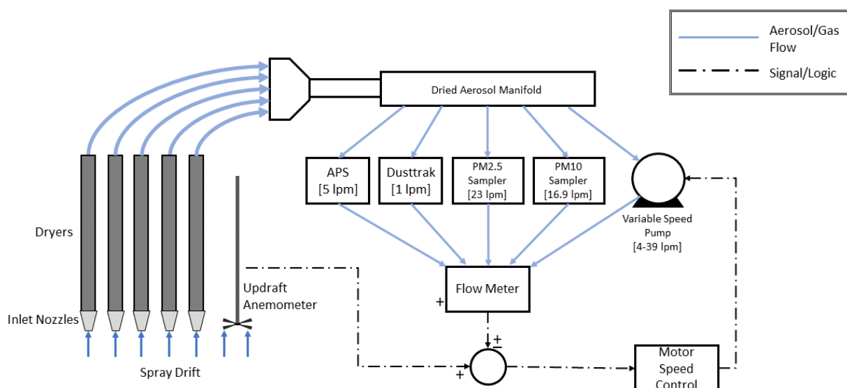
Figure 3. Feedback control for matching vertical updraft velocity.
