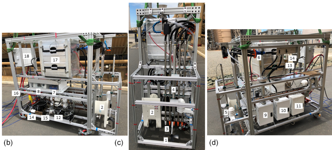
Figure 1. Sampling instrumentation package (a) diagram, (b) right side, (c) sampling end, and (d) left side.
