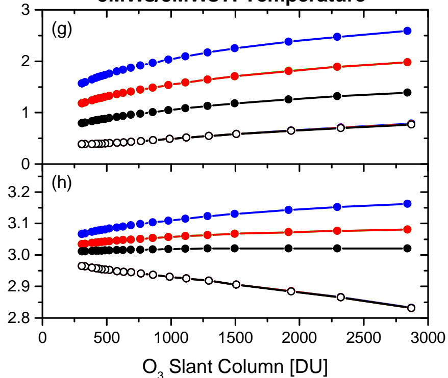
5MWs/5MWsT: Temperature
