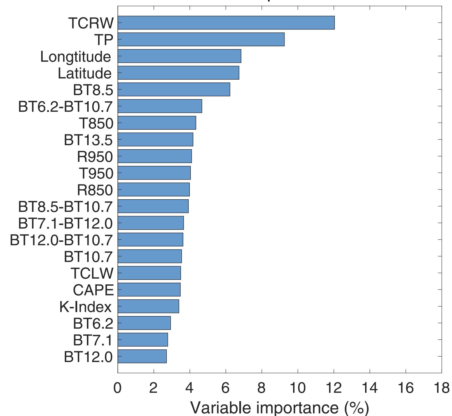
The variable importance of F4-IM
