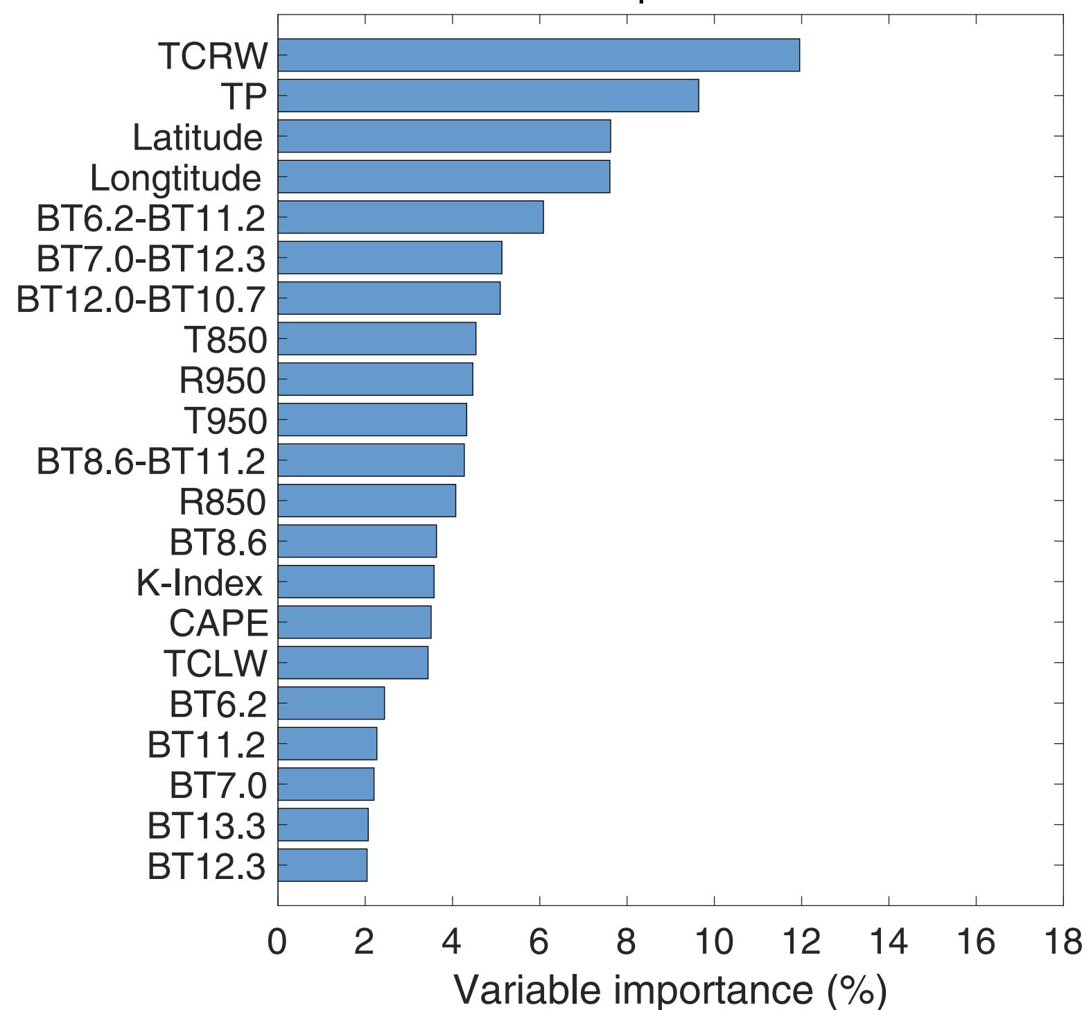
The variable importance of H8-IM
