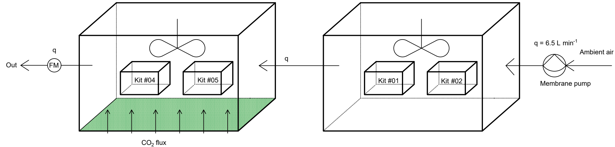
Flux chamber, opened bottom
