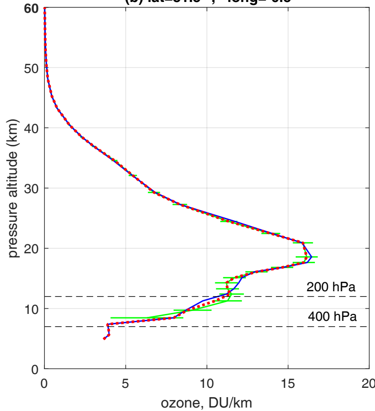
(b) lat=81.5°, long=-0.5°
