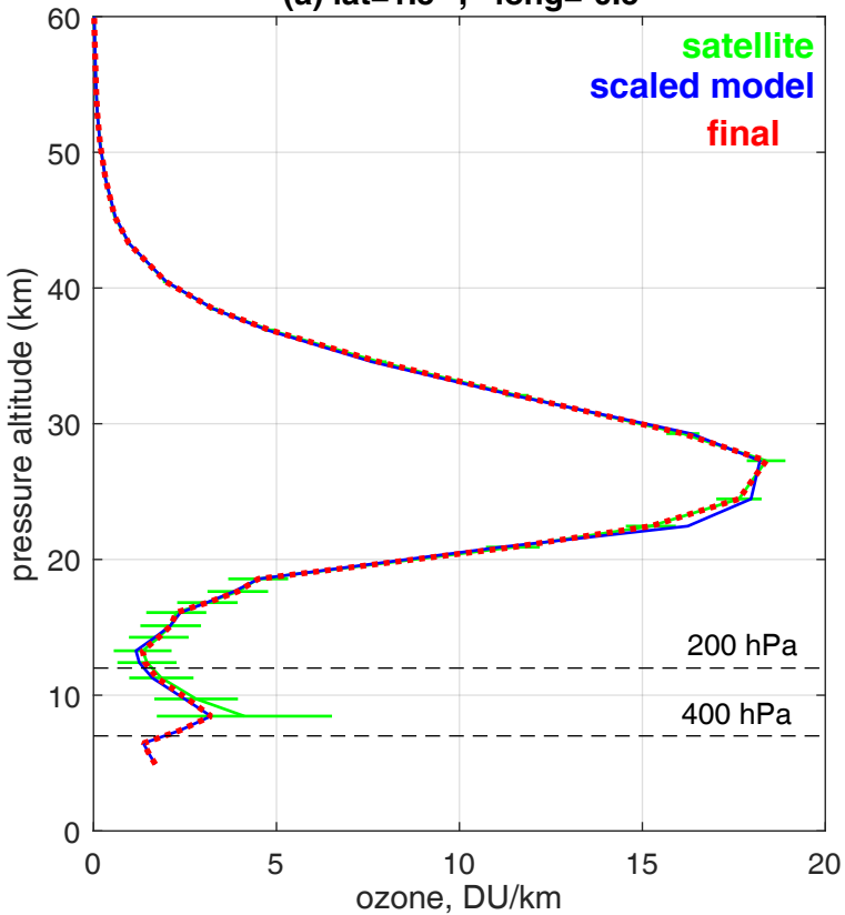
(a) lat=1.5°, long=-0.5°
