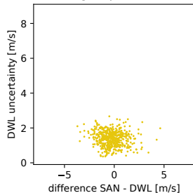
(c) DWL gust peaks \geq 14 m/s
