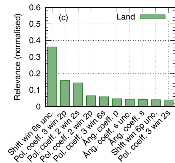
GOSAT XCH4
