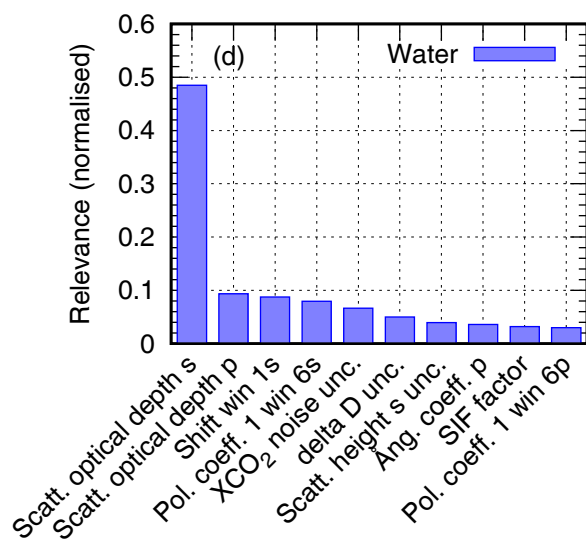
GOSAT XCH4
