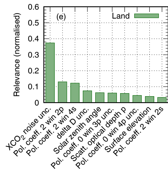
GOSAT XCH4 Proxy
