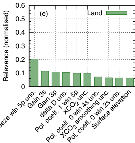
GOSAT-2 XCH4 Proxy
