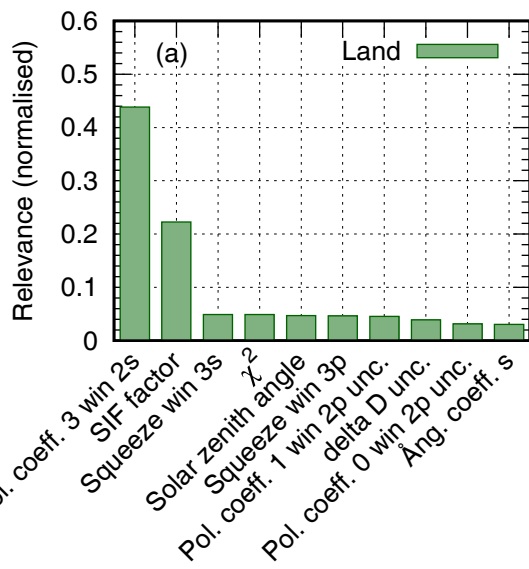
GOSAT-2 XCH4
