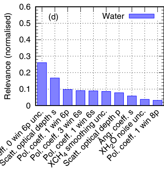
GOSAT-2 XCH4
