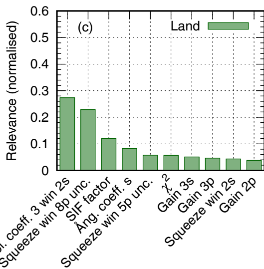
GOSAT-2 XCH4
