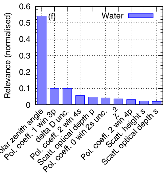
GOSAT-2 XCH4 Proxy
