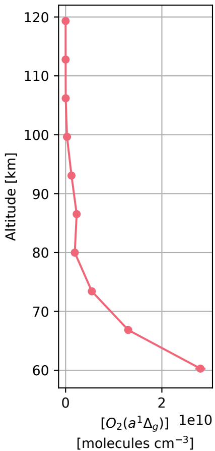
(a) Excited O_2
