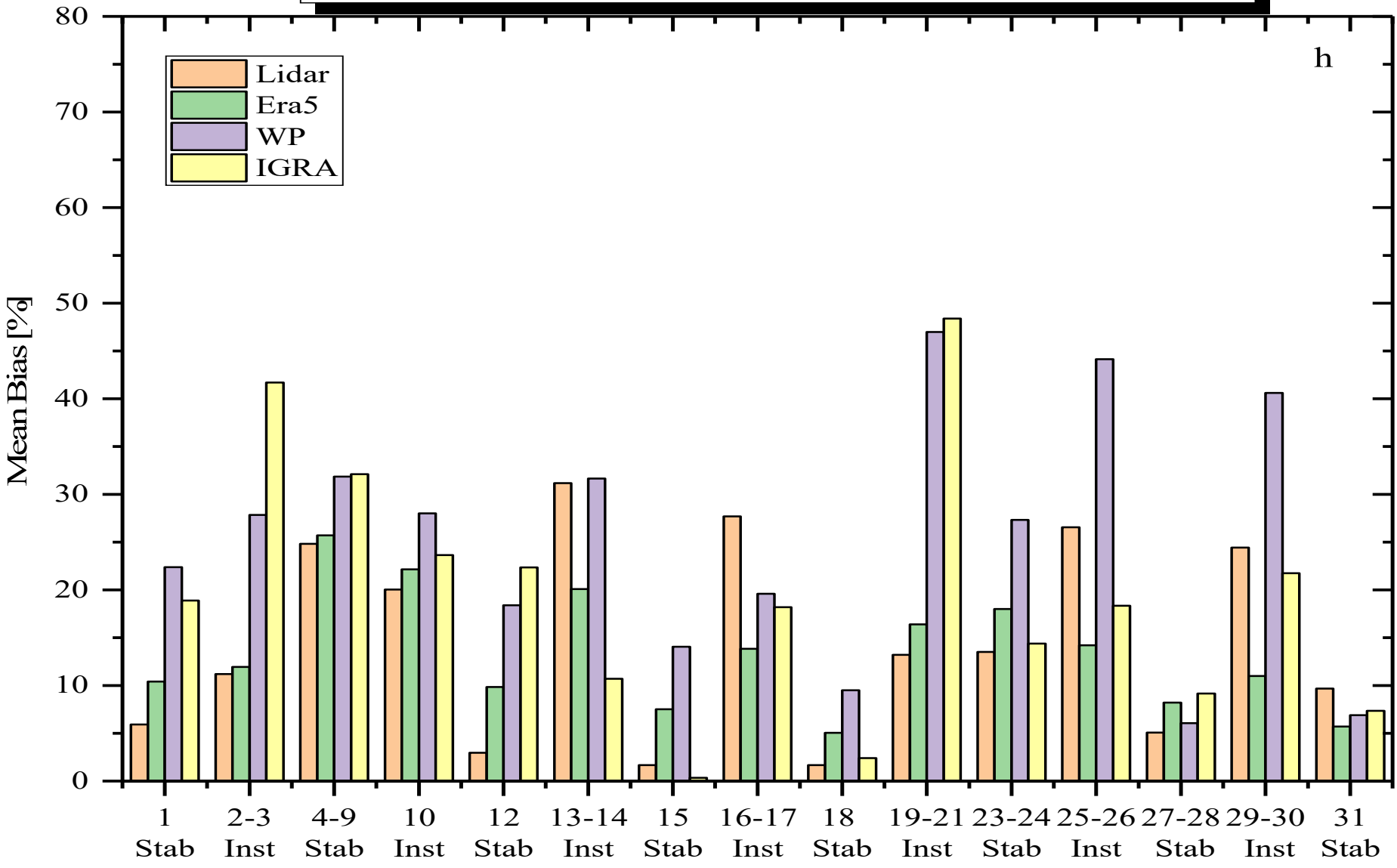
Max average bias [%] for each instrument used during measurements campaign
