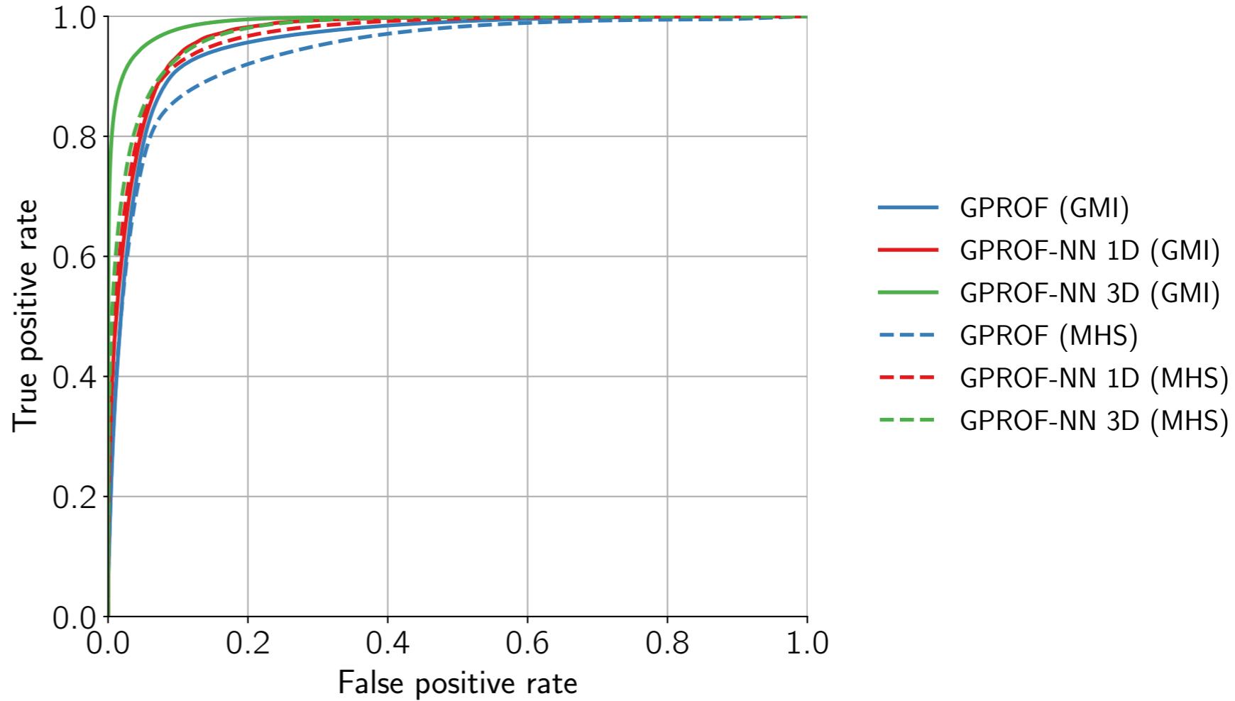
(b) ROC curve
