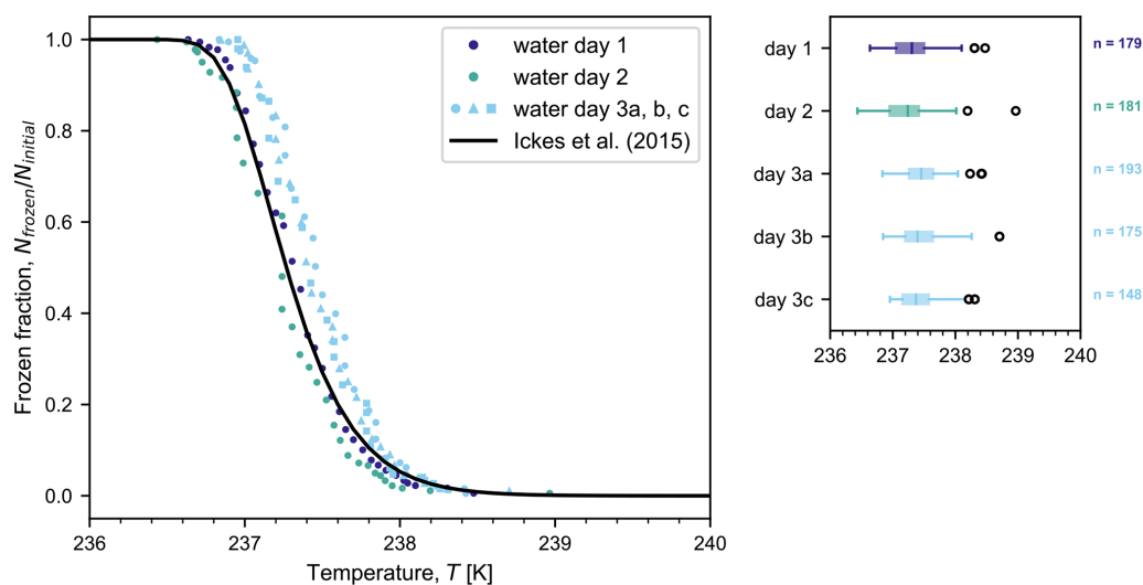
Figure 3. Frozen fraction of pure water (Sigma-Aldrich) droplets (with diameters as indicated in Table 1) as a function of temperature for different droplet populations (with n number of droplets) cooled at a rate of 1 \text{ K min}^{-1} on three separate days. The droplet population on day 3 was subjected to three freeze–thaw cycles (a, b, c). Also shown is the frozen fraction curve for the homogeneous freezing of water using the parameterization from Ickes et al. (2015) for droplets with a diameter of 75 \mu\text{m} . Box plots on the right-hand side summarize the experimental results. The centre line of each box plot indicates the median freezing temperature, the box spans the interquartile range (between the 25th and 75th percentiles), the whiskers extend to the maximum and minimum temperatures, and outliers are shown by open circles. The temperature accuracy of our measurements is estimated to be \pm 0.2 \text{ K} .
