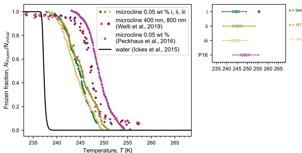
Figure 4. Frozen fraction of microcline droplets (0.05 wt % in SA water with diameters as indicated in Table 2) as a function of temperature for three independent droplet populations (i, ii, and iii with n number of droplets) cooled at a rate of 1 \text{ K min}^{-1} . We show frozen fractions reported by (i) Welti et al. (2019) obtained with the same microcline sample but using the Zurich Ice Nucleation Chamber (ZINC) for single particles size-selected to a mobility diameter of 400 or 800 nm and (ii) Peckhaus et al. (2016) for a suspension of 0.05 wt % microcline (digitized; P16 in the box plot). We emphasize that the total particle surface area in each case must be considered when comparing frozen fractions. The frozen fraction calculated using the parameterization from Ickes et al. (2015) for pure water droplets with a diameter of 75 \mu\text{m} is also shown. On the right, a box plot compares the freezing temperatures of the three droplet populations; the centre line indicates the median freezing temperature, the box spans the interquartile range (between the 25th and 75th percentiles), the whiskers extend to the maximum and minimum temperatures, and outliers are shown by open circles. The temperature accuracy of our measurements is estimated to be \pm 0.2 \text{ K} .
