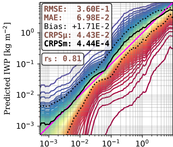
VISIR
