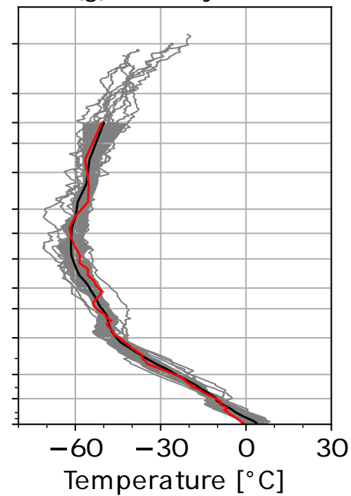
(g) DJF:Daytime
