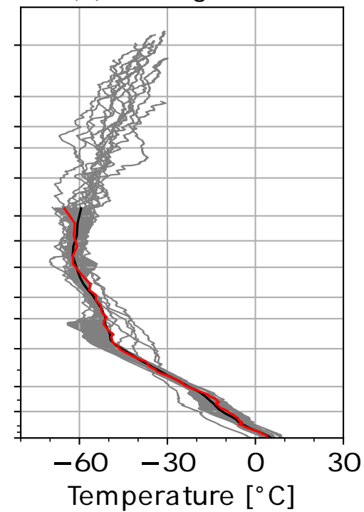
(h) DJF:Nighttime
