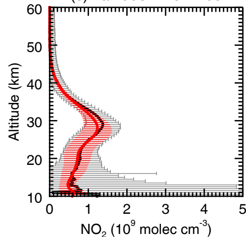
(c) Latitude: 20^{\circ} - 60^{\circ}
