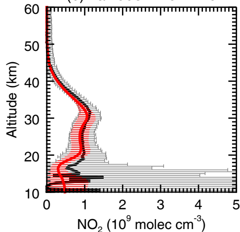
(b) Latitude: -20^{\circ} - 20^{\circ}
