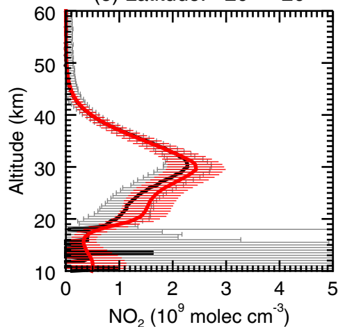
(e) Latitude: -20^{\circ} - 20^{\circ}
