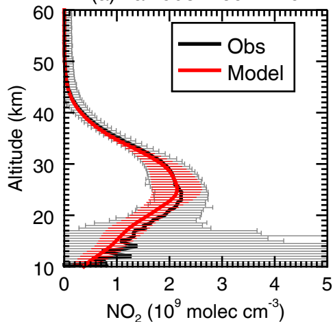
(a) Latitude: -60^{\circ} - -20^{\circ}
