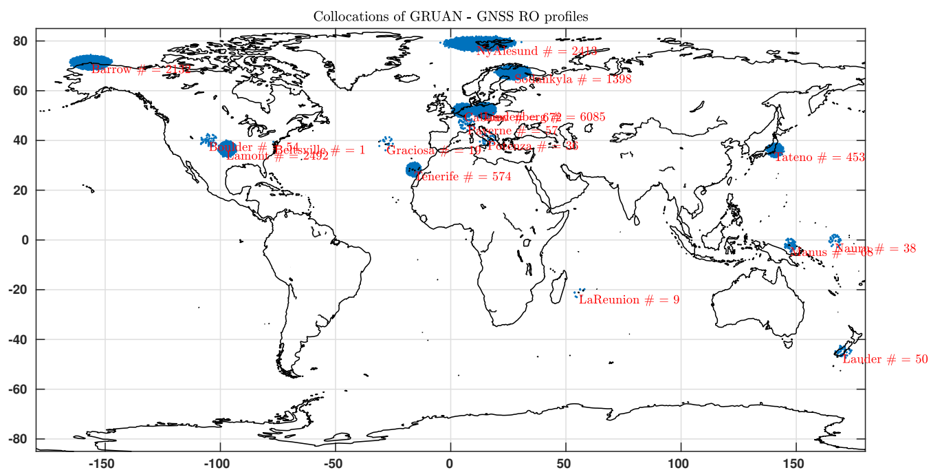
Figure S1. Map showing locations of the selected GRUAN RS92 sondes.
