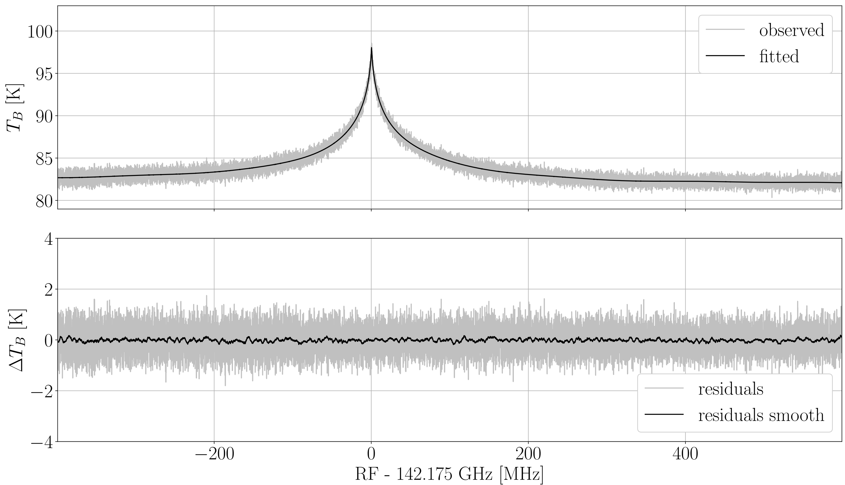
SOMORA O 3 spectrum: 2017-01-09 14:30
