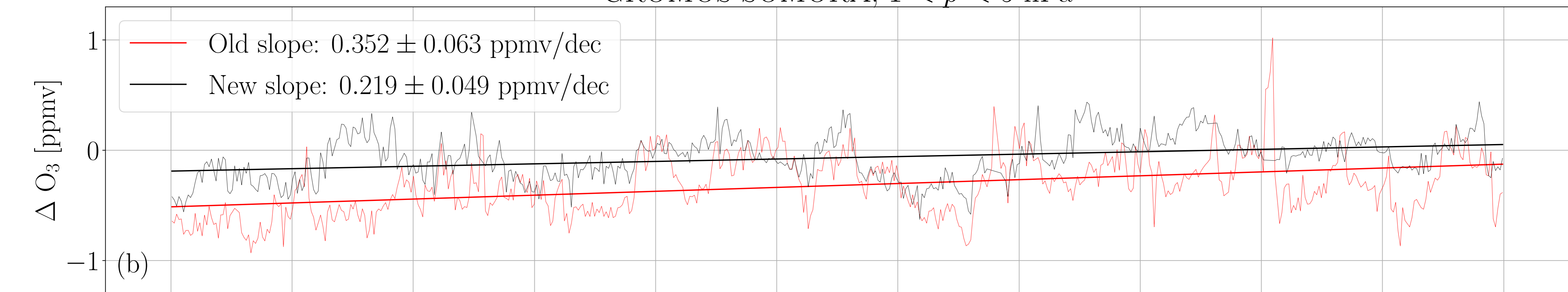
GROMOS-SOMORA, 1 < p < 5 hPa
