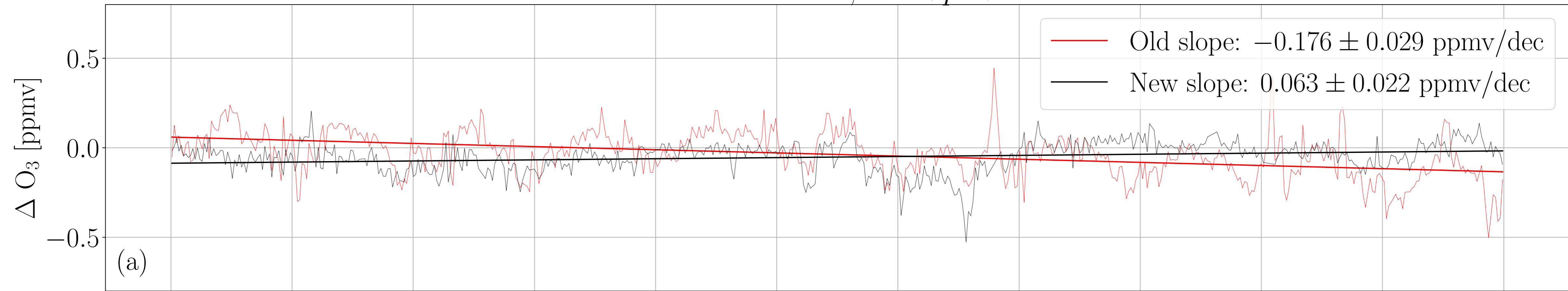
GROMOS-SOMORA, 0.1 < p < 0.9 hPa
