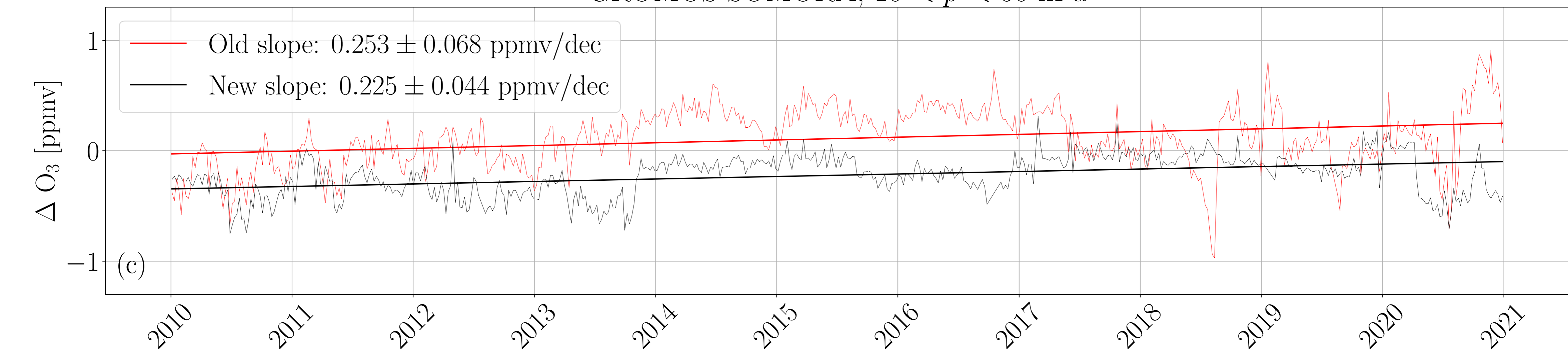
GROMOS-SOMORA, 10 < p < 50 hPa
