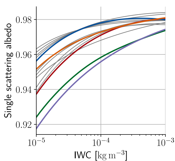
(e) Single scattering albedo (325 GHz)
