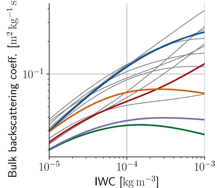
(c) Backscatter (94 GHz)
