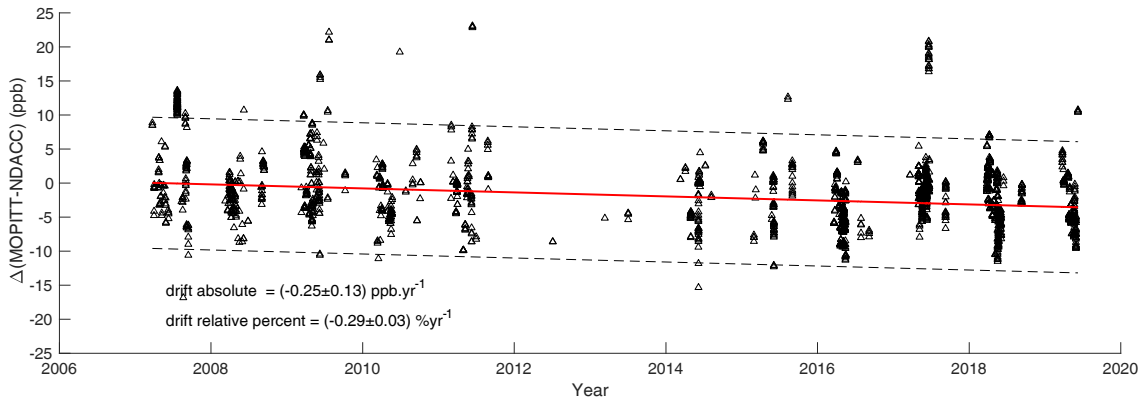
(a) NDACC
