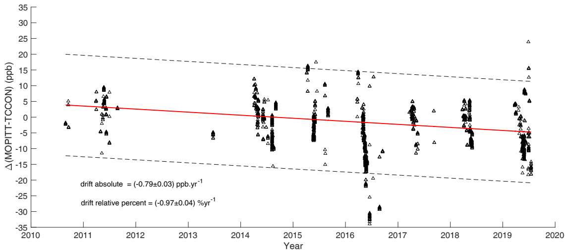
(b) TCCON
