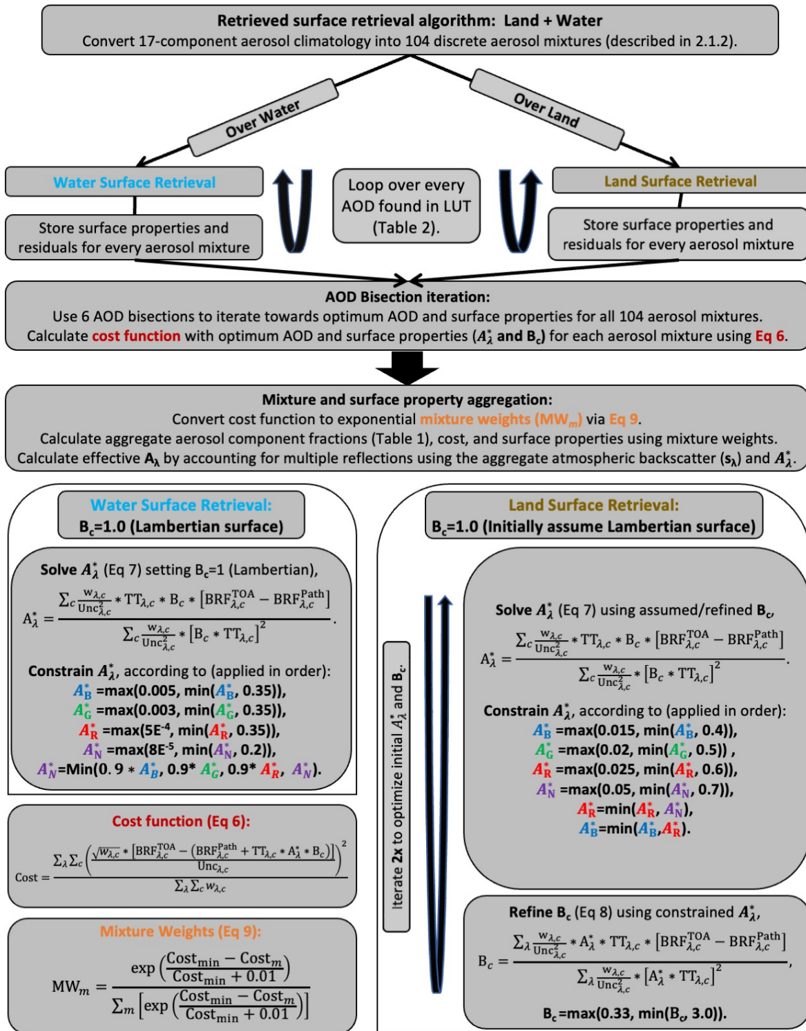
Figure S2) Flow chart of the MISR RA retrieved surface aerosol retrieval.
