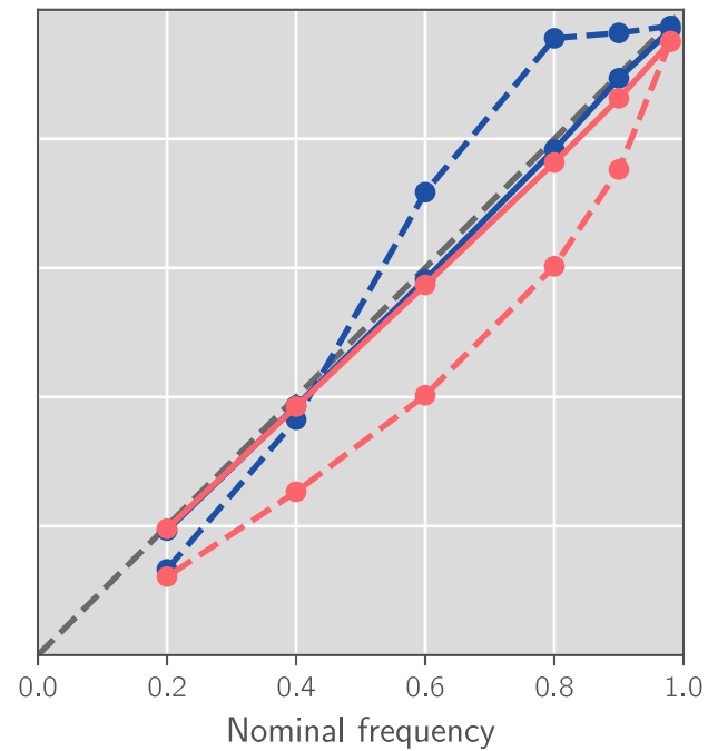
(c) Hydronn 2,All
