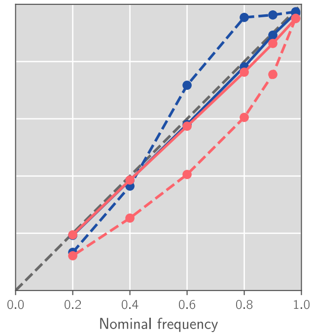
(b) Hydronn 4,All
