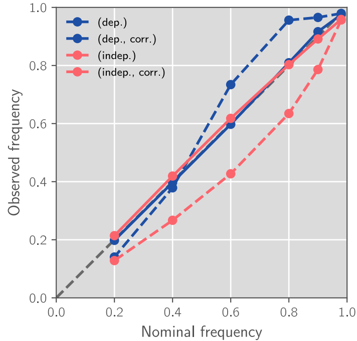
(a) Hydronn 4,IR
