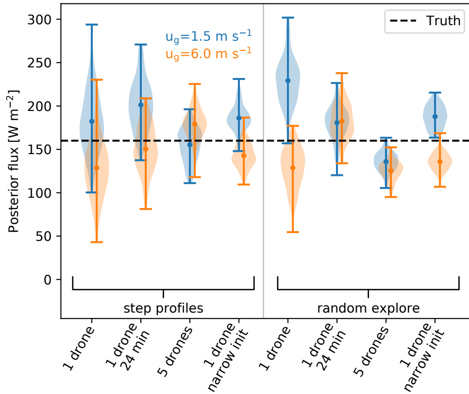
(a) Sensible heat flux
