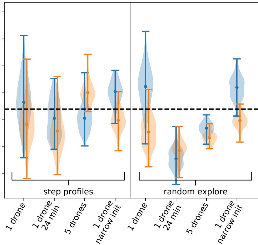
(b) Latent heat flux
