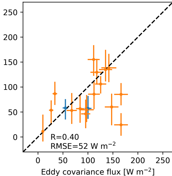
Latent heat flux
