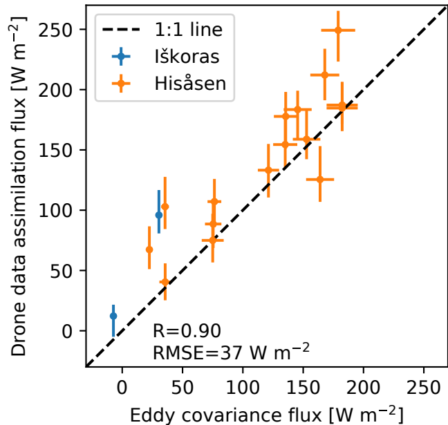
Sensible heat flux
