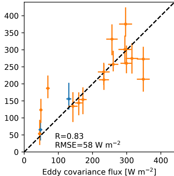
Sensible + latent heat flux
