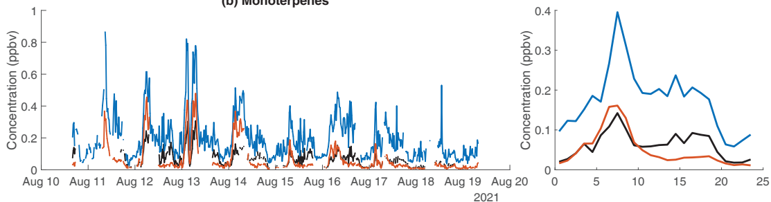
(c) Acetone
