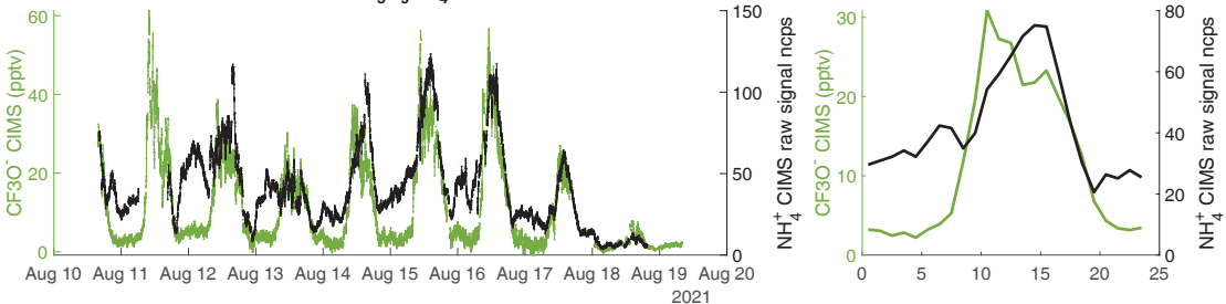
(c) C_5H_7NO_4
