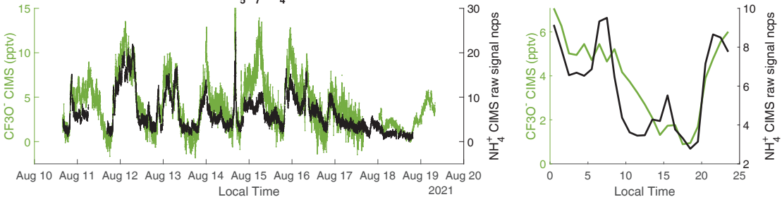
(c) C_5H_7NO_4
