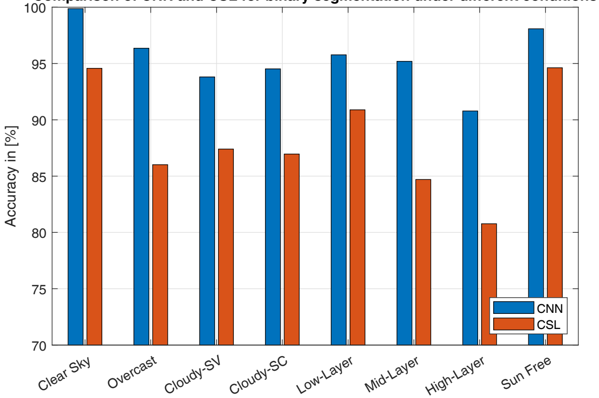
Comparison of CNN and CSL for binary segmentation under different conditions
