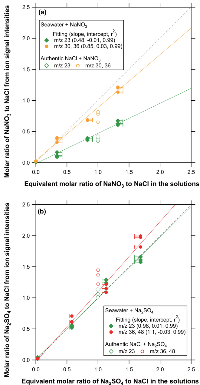
Figure 6. (a) Scatterplots of the molar ratios of SN to SC derived from ion signals versus the equivalent molar ratios of SN to SC in the solutions. The slope, intercept, and r^2 values for the linear regression are indicated in the legend. Solid and open symbols represent the data from seawater + SN and SC + SN particles, respectively. The error bars for the x axis represent the uncertainties in estimating the equivalent molar concentrations of the compounds (see the Supplement for details). (b) Same as (a) but for the molar ratios of SS to SC.
