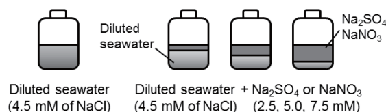
Figure 1. Summary of tested solutions. (a) Single-component solutions of NaNO 3 (SN), NaCl (SC), Na 2 SO 4 (SS), KNO 3 (PN), KCl (PC), and K 2 SO 4 (PS) with a molar concentration of 5 mM. (b) Multi-component solutions of NaNO 3 + NaCl + Na 2 SO 4 and KNO 3 + KCl + K 2 SO 4 with a molar concentration of 5 mM for each compound. (c) Diluted seawater (by a factor of 100; equivalent to 4.5 mM of NaCl) and diluted seawater with Na 2 SO 4 or NaNO 3 with molar concentrations of 2.5, 5.0, and 7.5 mM.
