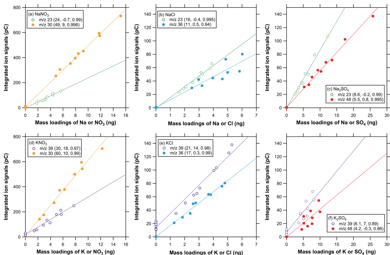
Figure 3. Scatterplots of integrated ion signals versus mass loadings (Na for m/z 23; K for m/z 39; \text{NO}_3 for m/z 30; Cl for m/z 36; \text{SO}_4 for m/z 48) for (a) SN, (b) SC, (c) SS, (d) PN, (e) PC, and (f) PS particles. The three values in the parentheses in the legend represent the slope, intercept, and r^2 , respectively, for the linear regression.
