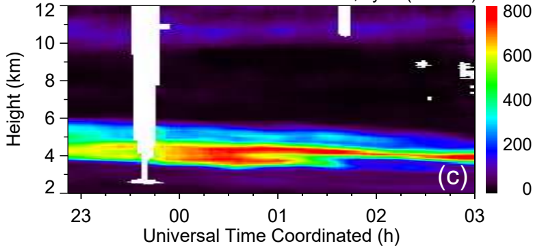
Fluorescence backscatter coefficient, cyan ( \text{Tm}^{-1} \text{sr}^{-1} )
