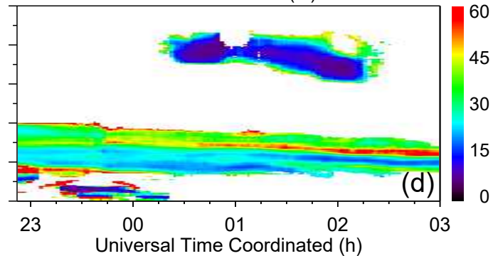
Particle lidar ratio (sr)
