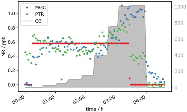
Acetaldehyde
