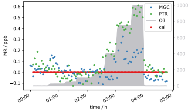
Acetaldehyde
