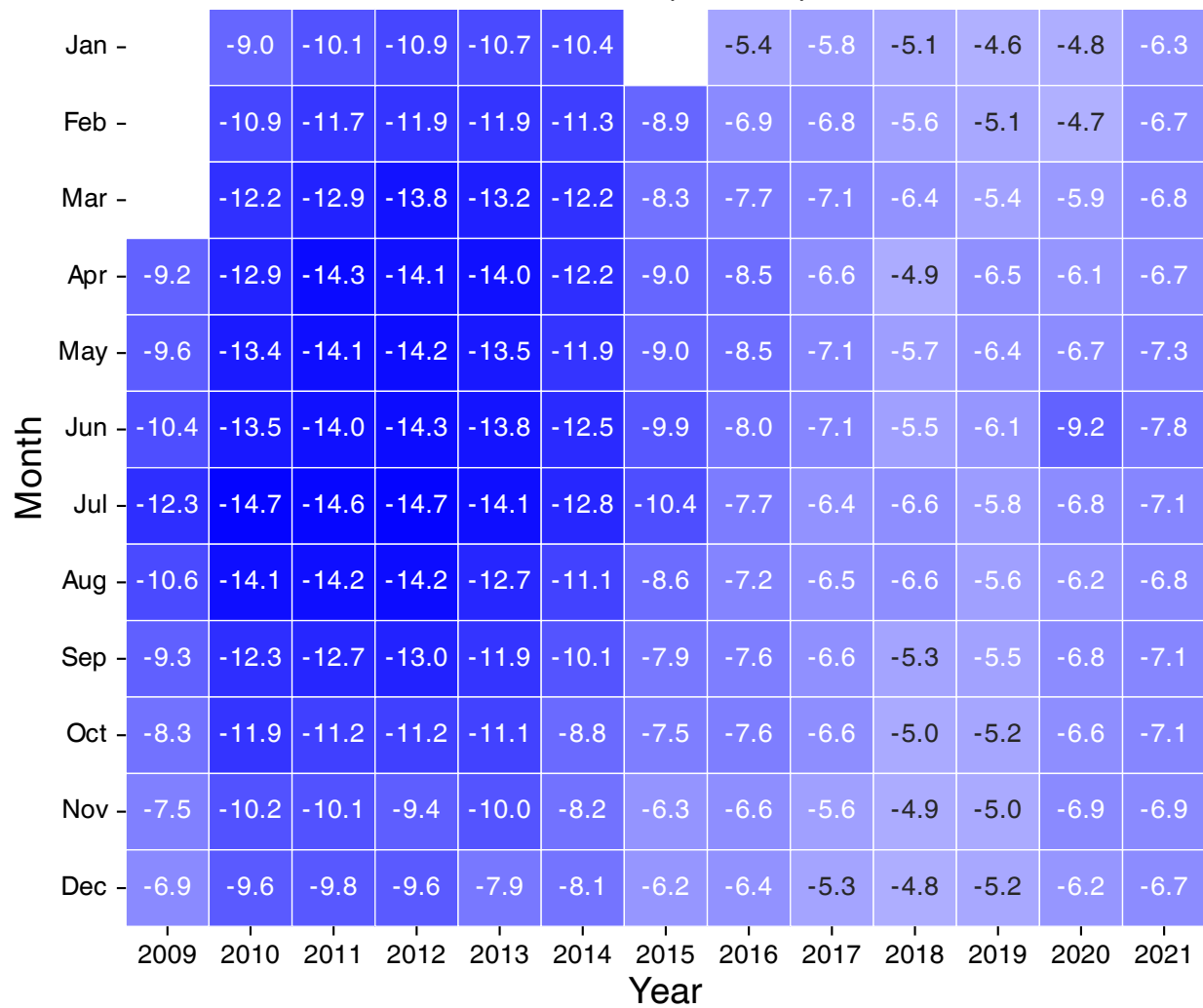
\Delta XCH_4 (Ocean)
