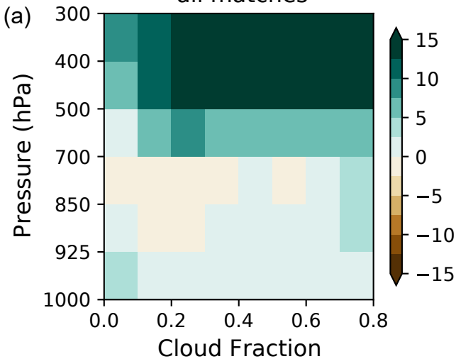
\Delta H 2 O Biases (% ppmv) day - all matches
