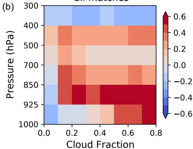
\Delta Temperature Biases (K) day - all matches
