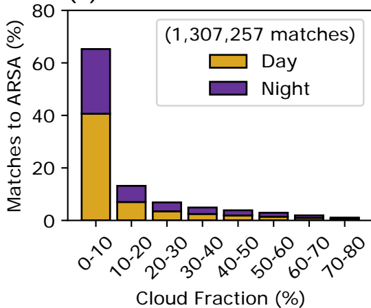
(c) 60°S to 30°S
