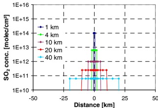
SO 2 scenario ,strong, 1' with 1 \cdot 10^{29} molecules in the plume SO 2 VCD
