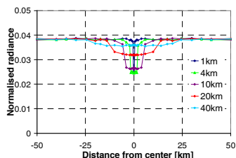
Radiance 313 nm
