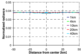
Radiance 313 nm
