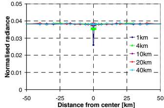
Radiance 313 nm
