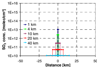
SO 2 scenario ,strong, 1' with 1 \cdot 10^{29} molecules in the plume SO 2 VCD
