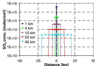
SO 2 scenario ,strong, 4' with 4 \cdot 10^{30} molecules in the plume SO 2 VCD
