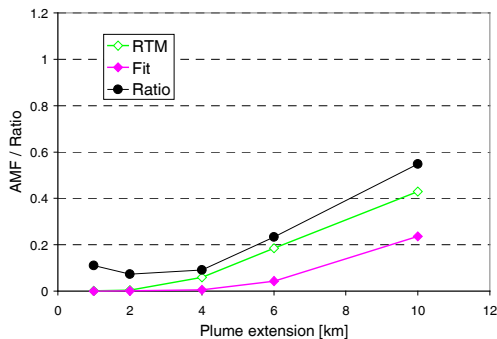
(e) 332 nm, 4 \cdot 10^{30} molecules
