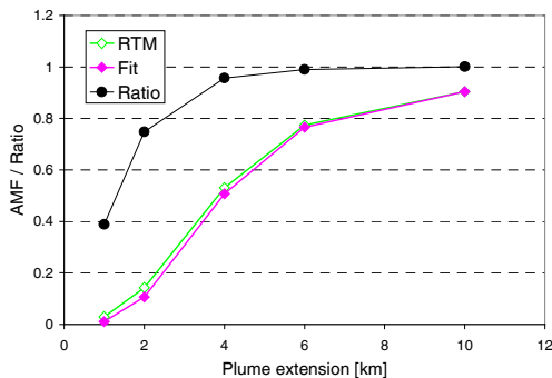
(e) 332 nm, 4 \cdot 10^{30} molecules
