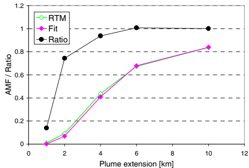
(c) 313 nm, 1 \cdot 10^{30} molecules
