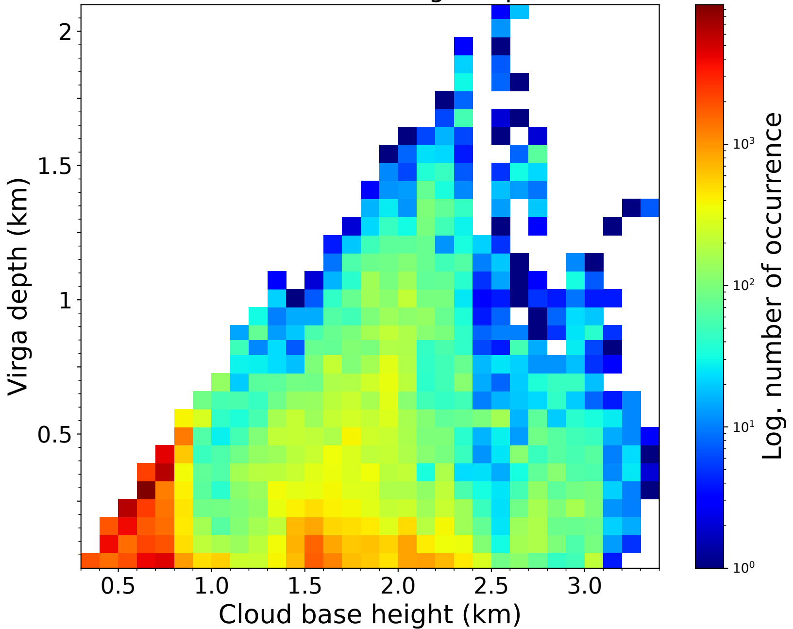
Ceilometer Cloud Base and Virga Depth Distribution
