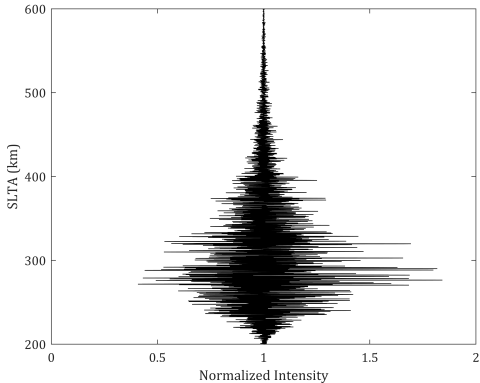
(a) Normalized intensity at the rightmost phase screen (observational plane).
