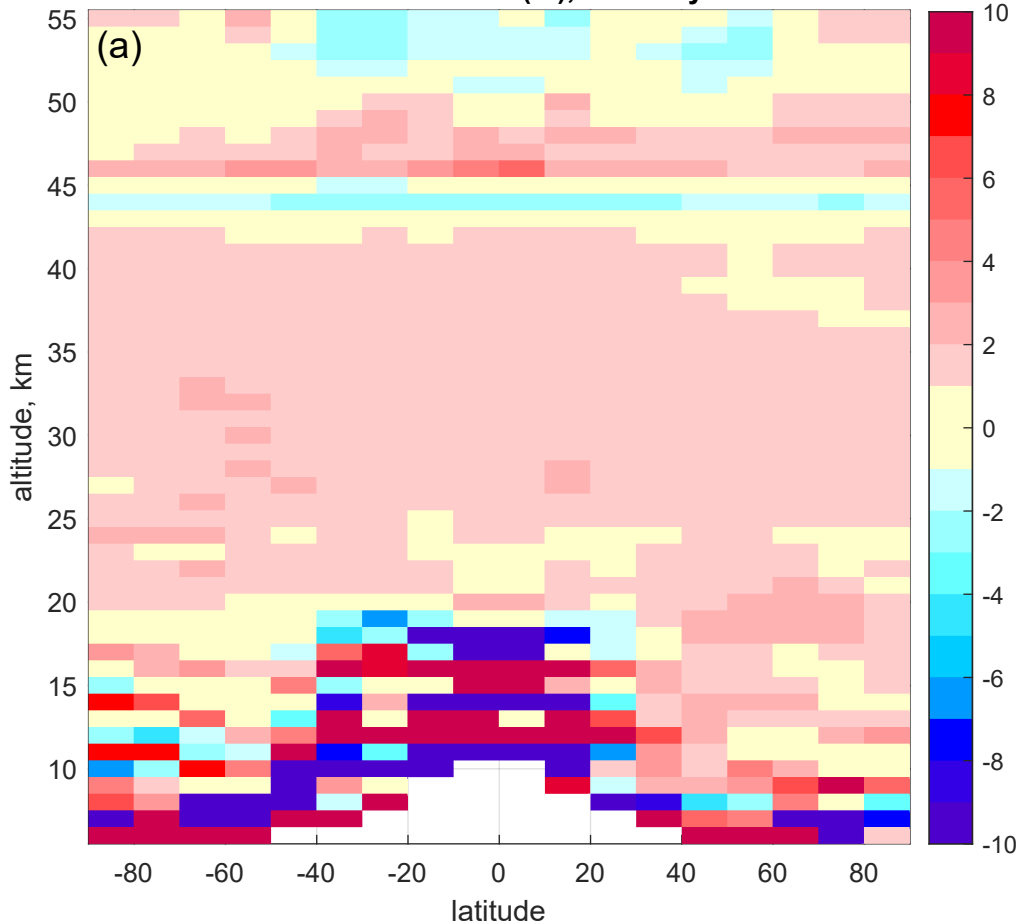
MIPAS v8 - MIPAS v7 (%), January 2008
