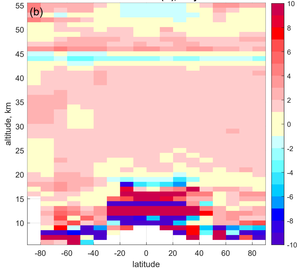
MIPAS v8 - MIPAS v7 (%), July 2008
