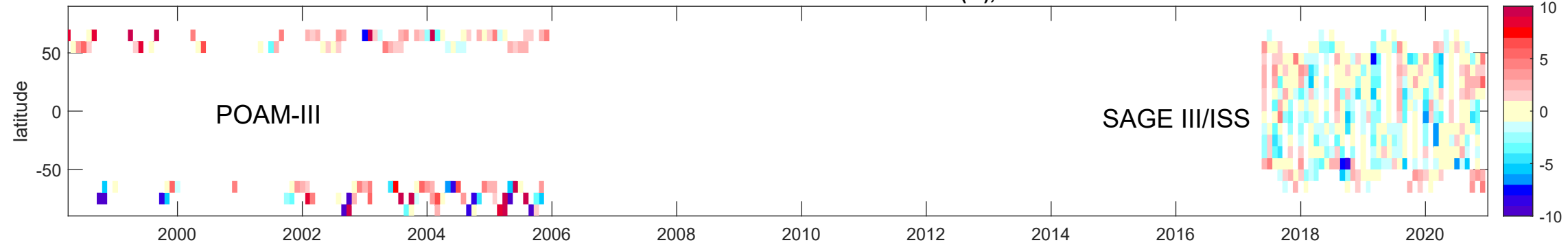
POAM-III and SAGE III/ISS minus SAGE-CCI-OMPS(%), 40 km
