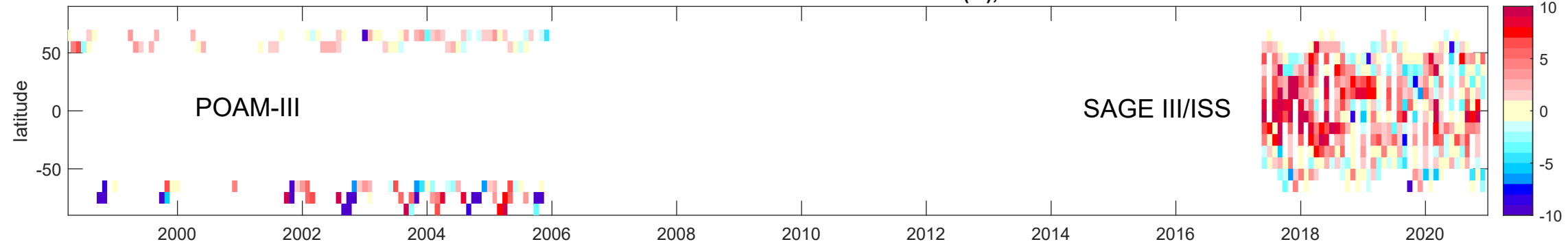
POAM-III and SAGE III/ISS minus SAGE-CCI-OMPS(%), 30 km
