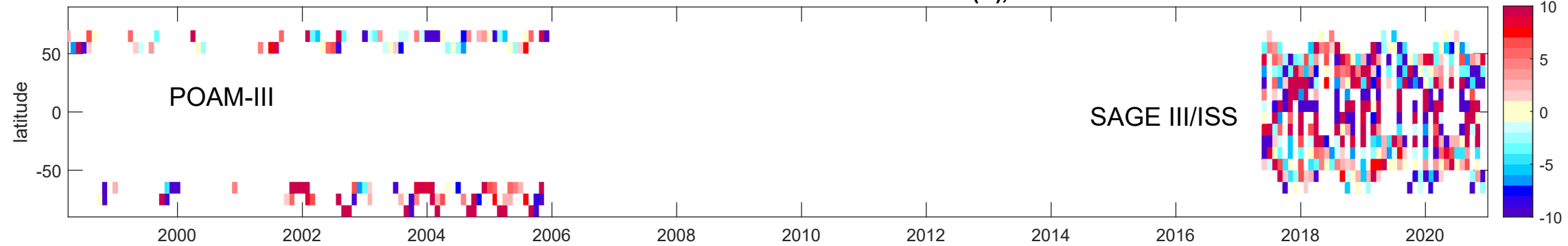
POAM-III and SAGE III/ISS minus SAGE-CCI-OMPS(%), 20 km
